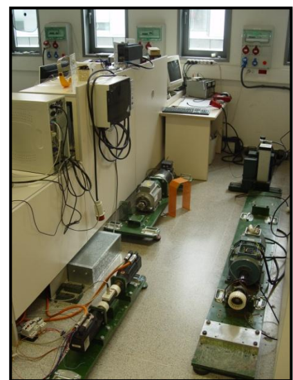
PMSM Experimental Bench
